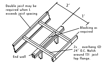
O GABLE END OVERHANG
