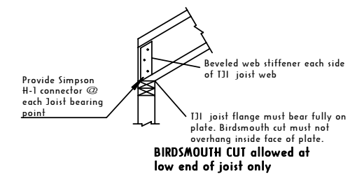
BC ROOF JOIST @ BEARING WALL
