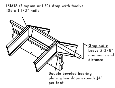
R14 RIDGE DETAIL
