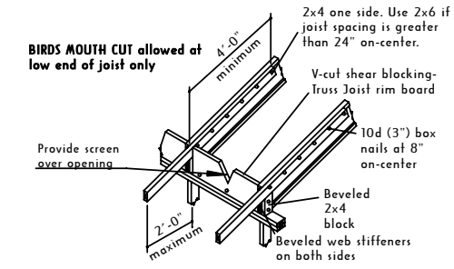
R9 EVE OVERHANG
