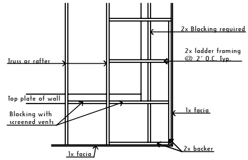
Typ. Gable End Framing @ Eave
