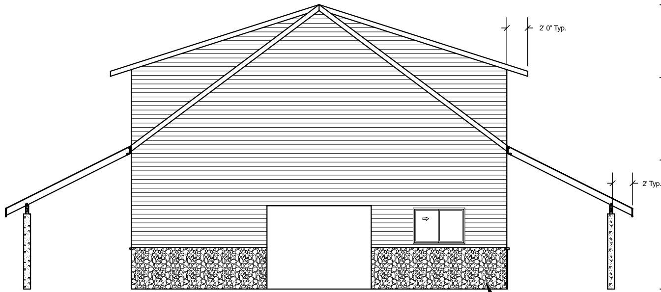
D 3 ELEVATION
