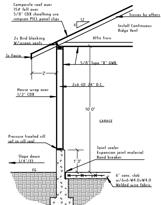
1 TYP. GARAGE WALL Scale 1/2" = 1'-0"
