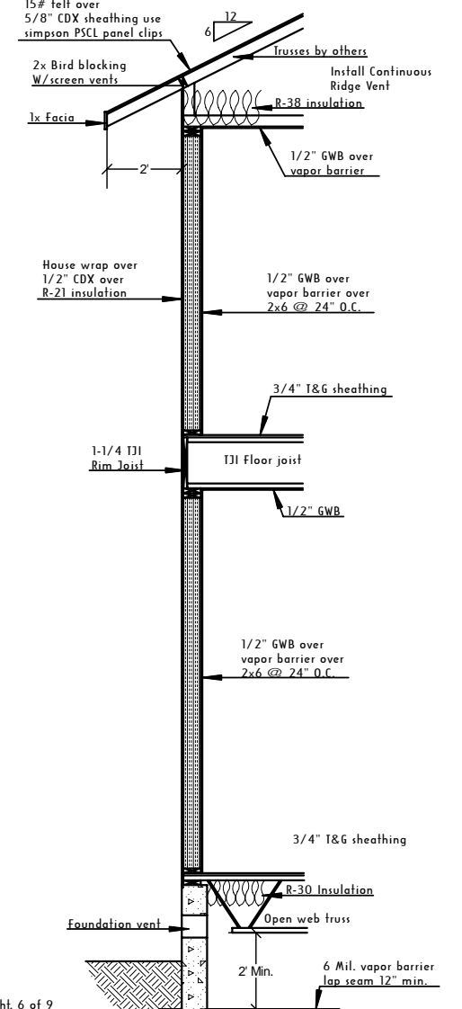
3 TYP. EXT. WALL Scale 1/2" = 1'-0"
