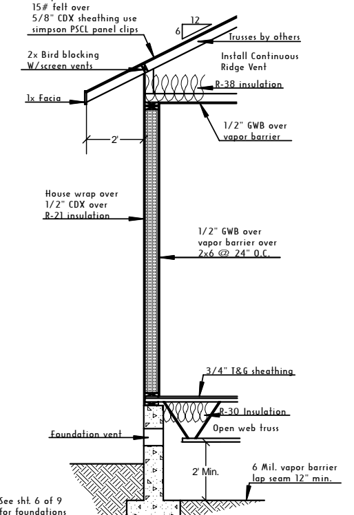
2 TYP. EXT. WALL Scale 1/2" = 1'-0"
