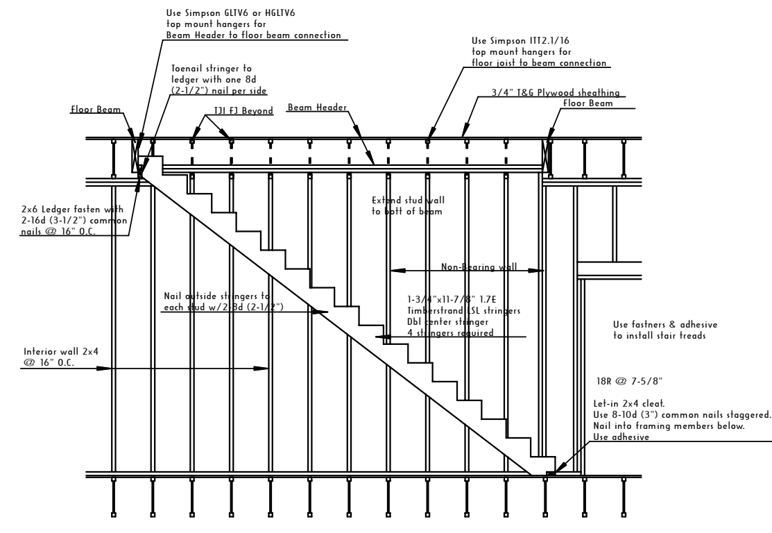
6 STAIRS 2nd FLOOR BEDROOM Scale 1/2" = 1'-0"
