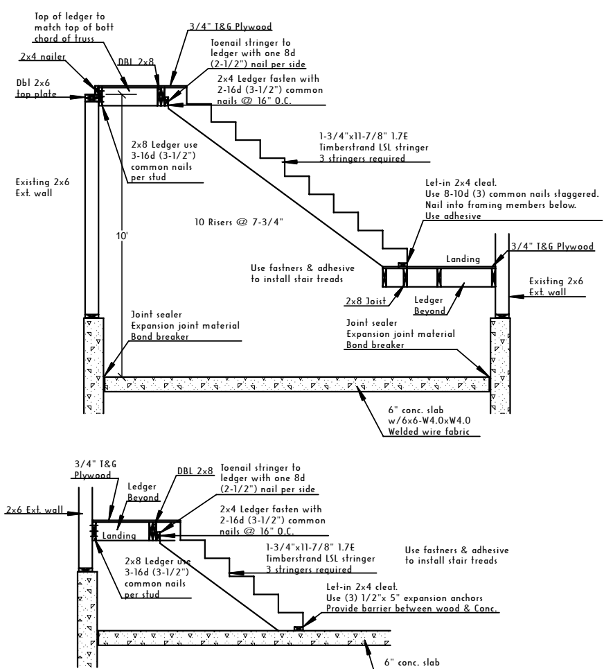
5 STAIRS GARAGE Scale 1/2" = 1'-0"
