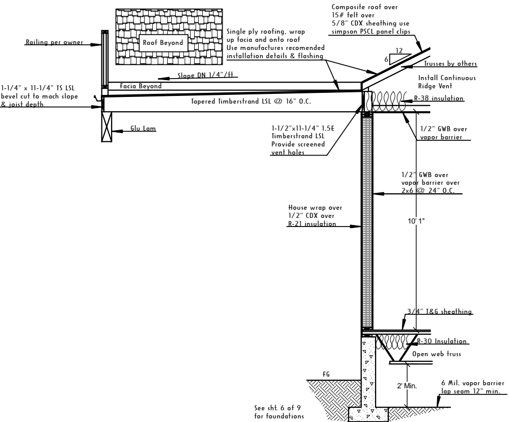
4 UPPER DECK Scale 1/2" = 1'-0"
